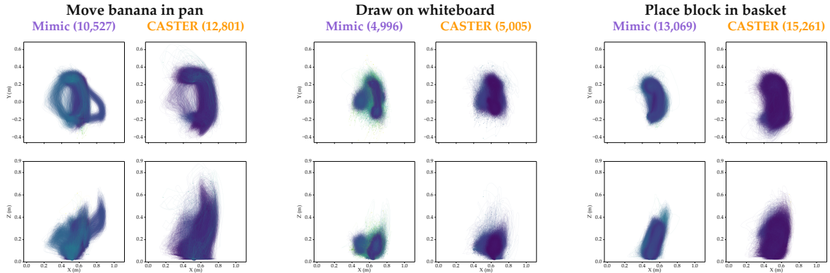
Fig. 5. End-effector trajectories from validated videos produced by CASTER and Mimic over the same set of 20 generated videos per task, shown in the X-Y (top) and X-Z (bottom) planes for three manipulation tasks. Parentheses indicate the number of feasible trajectories for each method. Darker colors indicate lower optimization cost.
